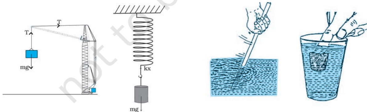
Fig. 4.9 Some examples of contact forces in mechanics.
